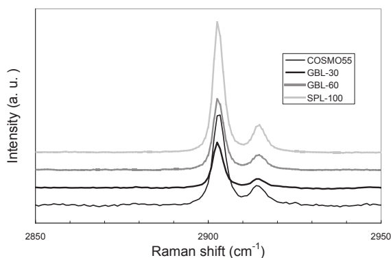
Figure 3. Raman spectra of C-H stretching mode of methane hydrate in glass beads.
