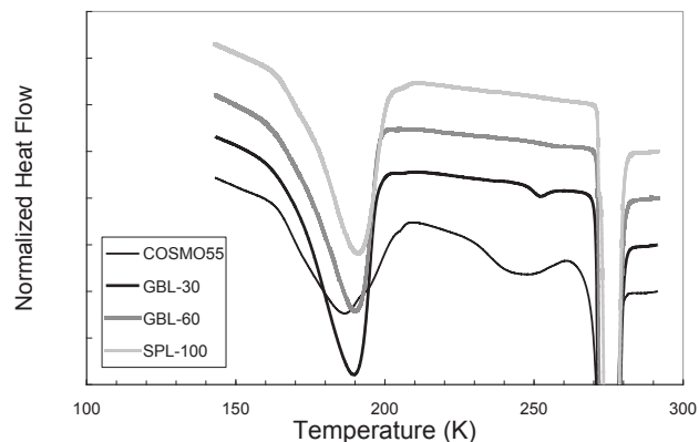
Figure 4. Thermograph shows the changes of heat flow. Negative direction of the normalized heat flow means endothermic.
