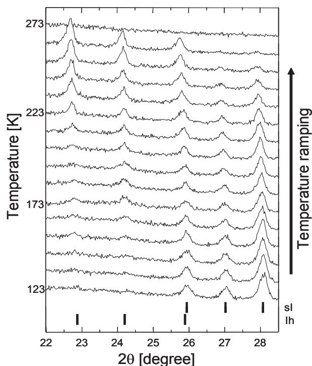
Figure 6. PXRD profiles in the dissociation process for the methane hydrate sample of COSMO55. The upper tick marks represent the peak positions for the structure I hydrate, and the lower represent hexagonal ice Ih.
