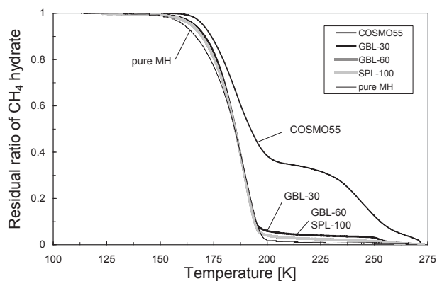
Figure 5. Residual ratio of methane hydrate in the sample plotted against temperature. GBL-60 is overlapped with SPL-100.
