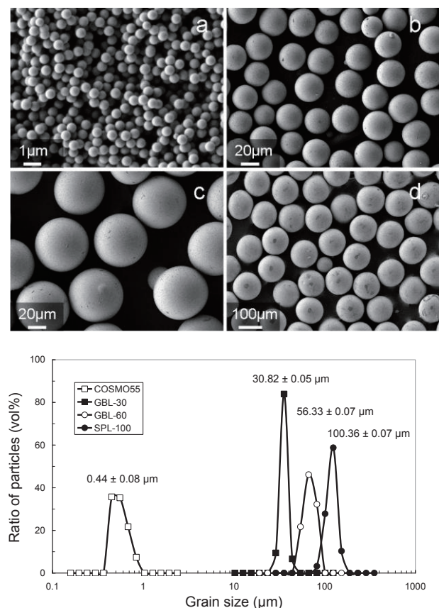
Figure 1. FE-SEM images of glass beads, size distributions, mean diameters and their standard deviations. (a) COSMO55, (b) GBL-30, (c) GBL-60, (d) SPL-100.
