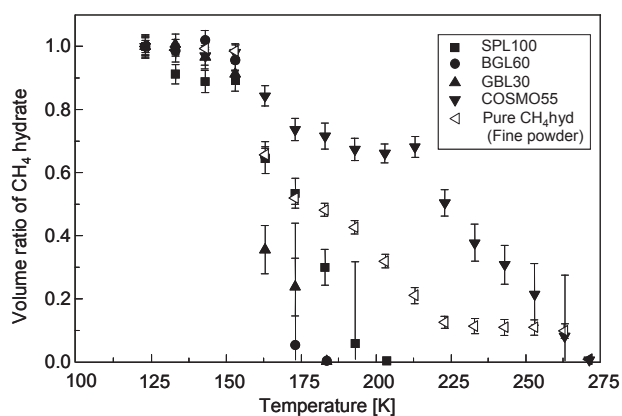
Figure 7. Volume ratio of methane hydrate in the sample by using PXRD data plotted against temperature.
