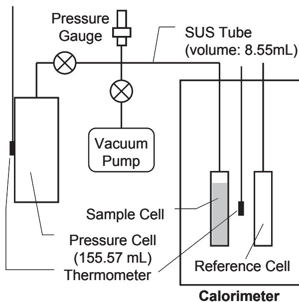
Figure 2. Schematic view of the calorimetric system.
