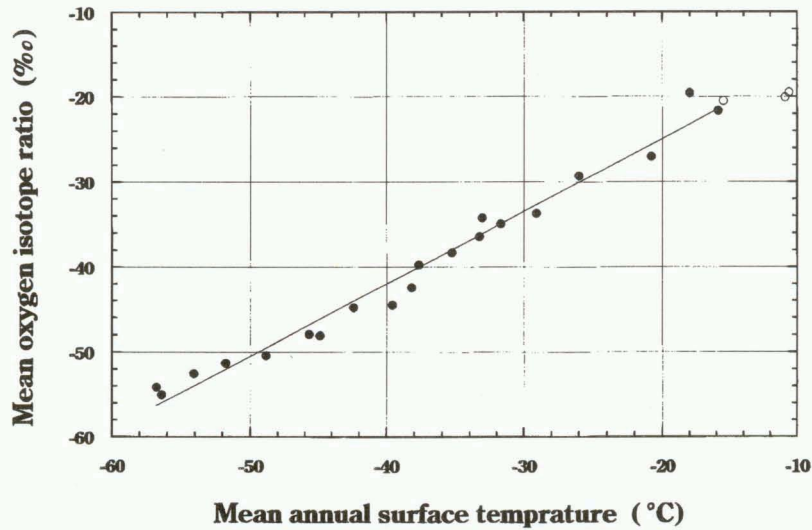
Fig. 3. Mean \delta^{18}O value of near-surface snow plotted against mean annual surface temperature (10 m-depth snow temperature) (after Satow et al. , 1999). The straight line is given by eq. (2). Three points on the coast marked by open circles are excluded from the regression equation.
