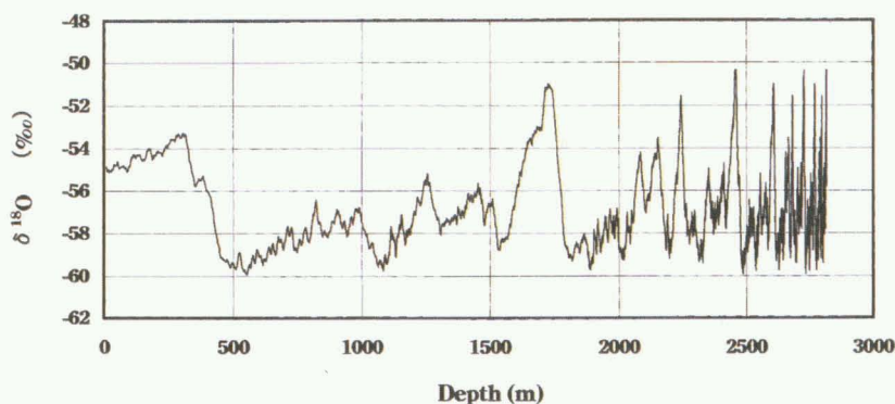
Fig. 12. Estimation of a glacial-interglacial \delta^{18}\text{O} cycle below a depth of 2500 m at Dome Fuji.
