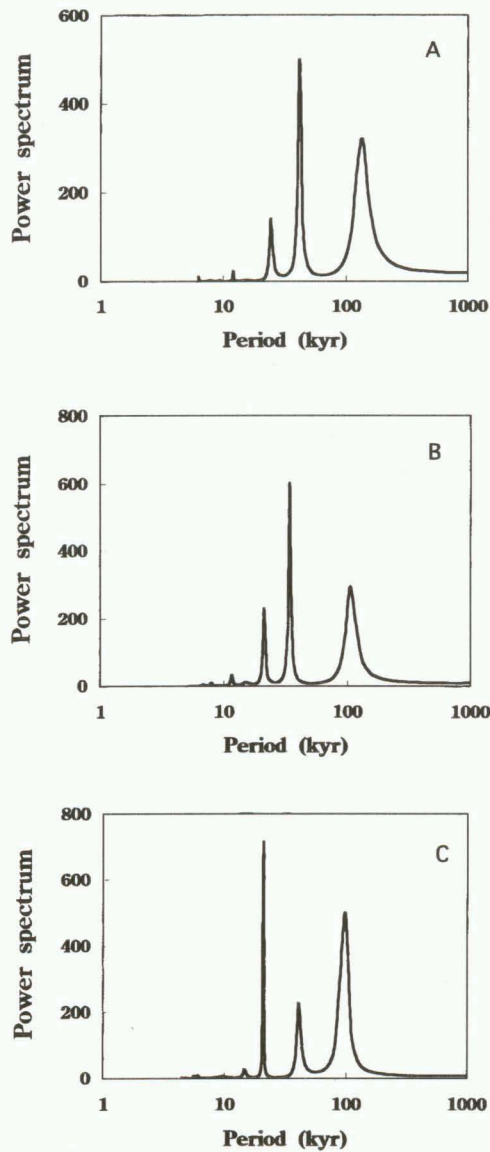
Fig. 10. Power spectrum for each glacial period in the Dome Fuji ice core. The power spectrum for the Wisconsin glacial period is shown in the upper figure (A); for the Illinoian period in the middle figure (B); for the Kansan glacial period in the lower figure (C). The vertical-axis unit is arbitrary.
