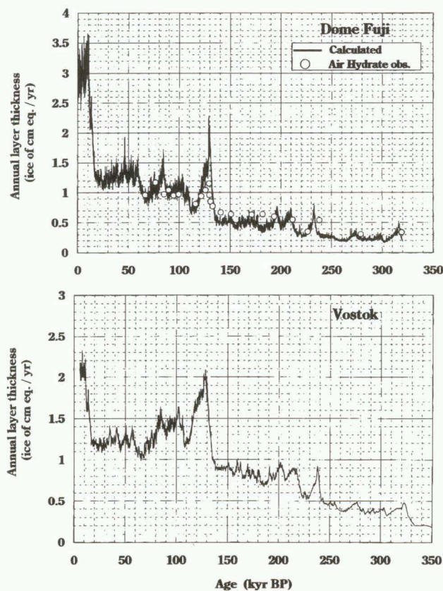
Fig. 11. Annual layer thickness profile, calculated (solid line) and estimated values from air hydrate measurements (circle) for Dome Fuji (top figure) and annual layer thickness profile calculated for Vostok (bottom figure).
