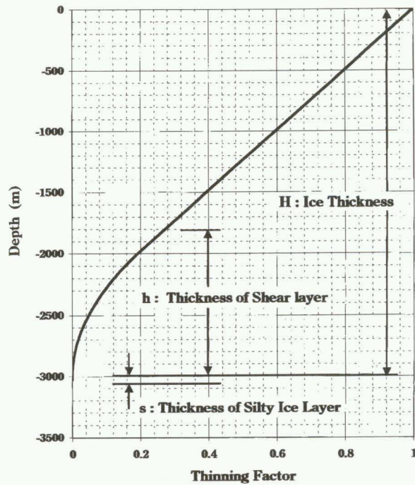
Fig. 5. Thinning factor for annual layer thickness calculated by the Dansgaard-Johnson model.
