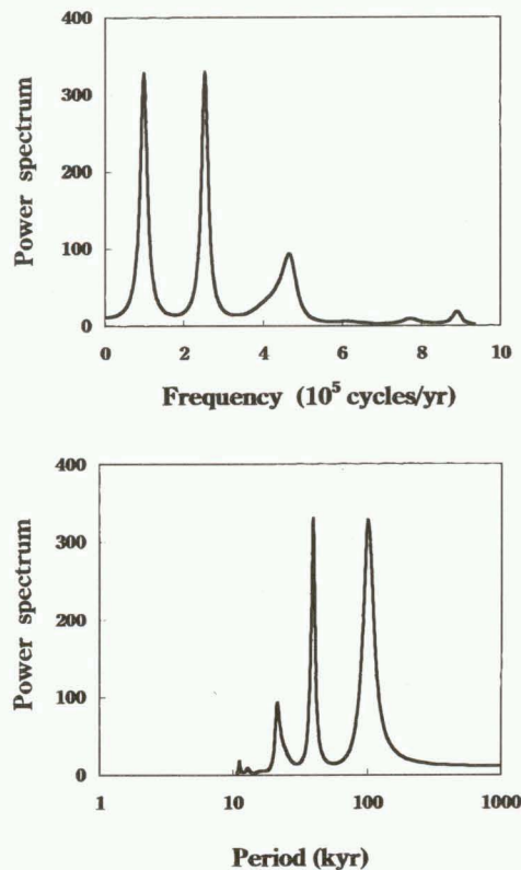
Fig. 9. Power spectrum of \delta^{18}\text{O} change for the 320 kyr Dome Fuji ice core. The top figure shows the spectral power versus the frequency, and the bottom figure shows the spectral power versus the period. The vertical-axis unit is arbitrary.
