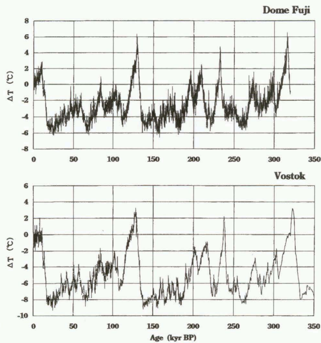
Fig. 8. Surface temperature variations at Dome Fuji and Vostok. Temperature difference \Delta T at Dome Fuji is calculated from eq. (5). \Delta T at Vostok is after Jouzel et al. (1996) and Petit et al. (1999).
