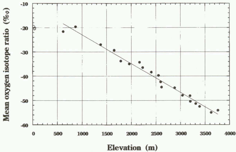
Fig. 2. Mean \delta^{18}O value of near-surface snow plotted against elevation (after Satow et al. , 1999). The straight line represents eq. (1).
