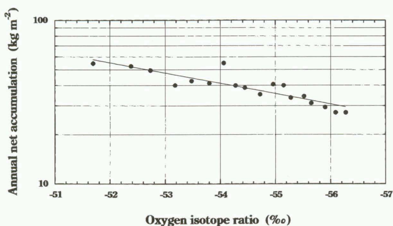
Fig. 4. The relationship between accumulation rate and mean \delta^{18}\text{O} value of near-surface snow (after Satow et al. , 1999). The straight line is given by eq. (3).
