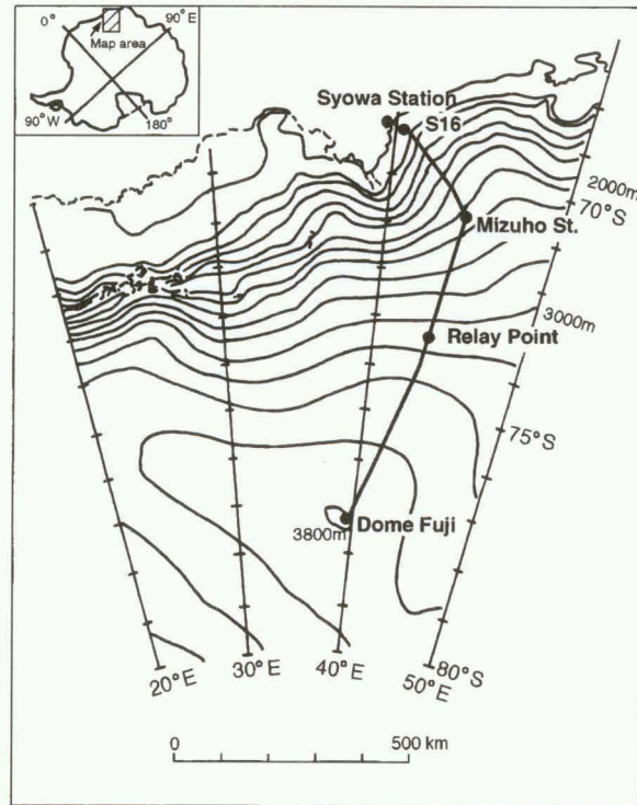
Fig. 1. Traverse route from Syowa Station to Dome Fuji Station.
