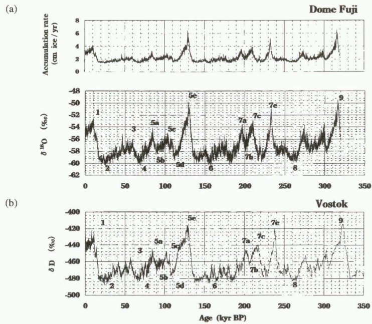
Fig. 7. (a) \delta^{18}O profile obtained at Dome Fuji. Accumulation rate, \lambda_0 is calculated from eq. (4). (b) \delta D profile obtained at Vostok (after Jouzel et al., 1996; Petit et al., 1999). MIS numbers are estimated and shown in both (a) and (b).
