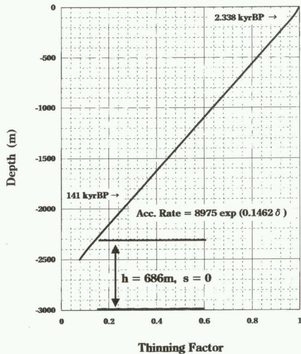
Fig. 6. Thinning factor profile obtained for the Dome Fuji core.
