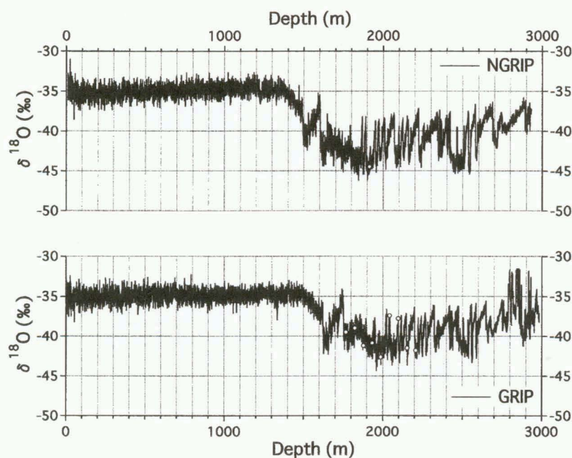
Fig. 1. \delta^{18}\text{O} profiles of GRIP and NGRIP ice cores. Open circles show sampling positions for this study.
