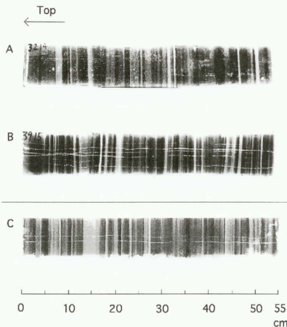
Fig. 2. Cloudy band stratigraphy. A. GRIP sample (Bag No. 3214, Depth 1767.15–1767.70 m), B. GRIP sample (Bag No. 3915, Depth 2152.70–2153.25 m), C. NGRIP sample (Bag No. 3480, Depth 1913.45–1914.00 m) White wavy lines along the core axis on the sample surface are scratched traces caused by a probe for ECM measurements.
