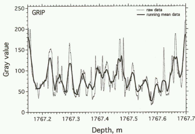
Fig. 4. Gray value profiles of raw data (dotted curve) and running mean data (solid curve) of a GRIP sample from a depth of 1767.15 m.
